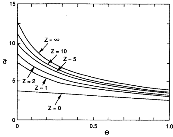
FIG. 1. The normalized conductivity as a function of the normalized temperature \Theta = T_e/(511 \text{ keV}) for various values of the effective ion charge state Z .
